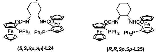
Scheme 16
