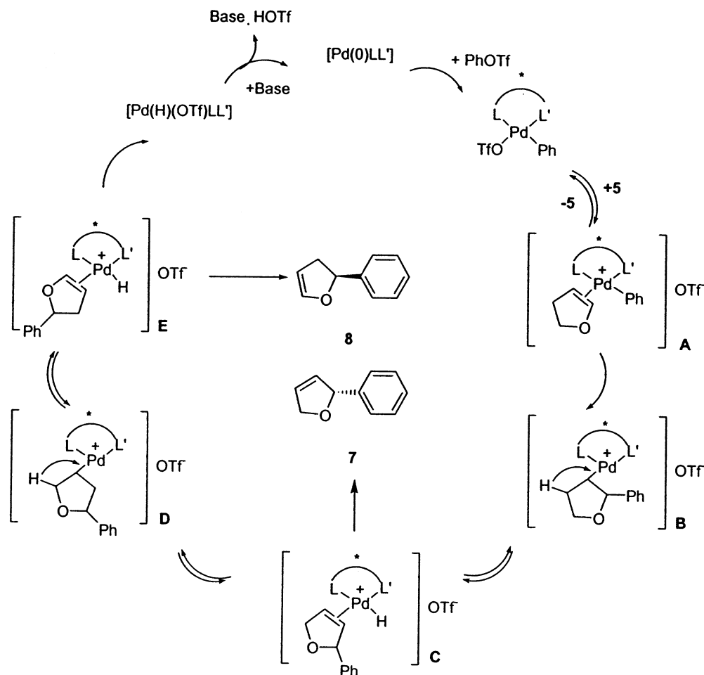
Scheme 17
