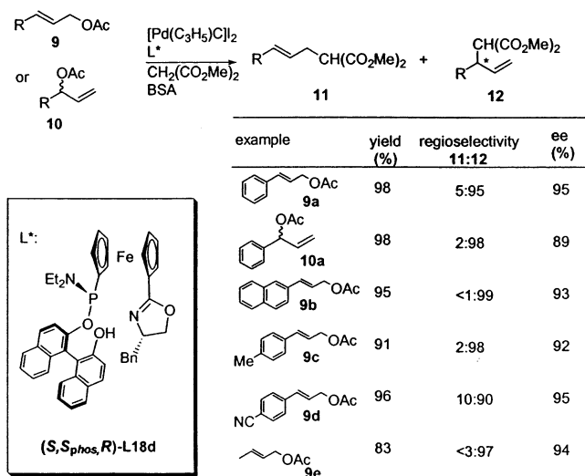
Scheme 12
